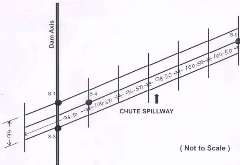
Holes proposed to be drilled at Spillway at Sapta Kosi High Dam Multipurpose Project
